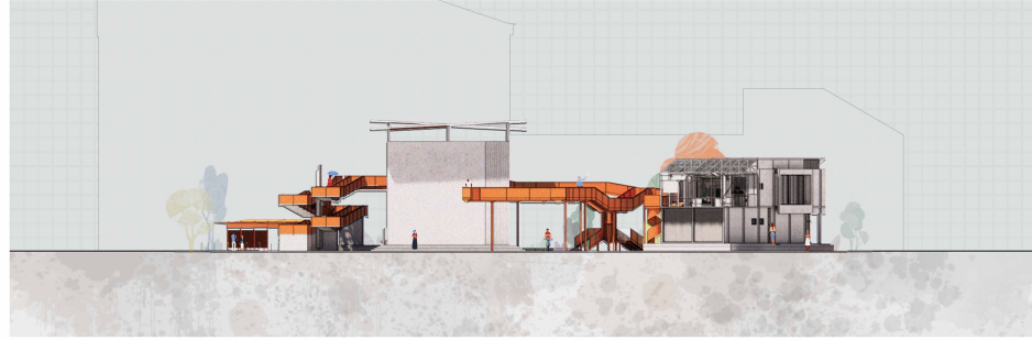
Right Elevation (south) scale 1:300
