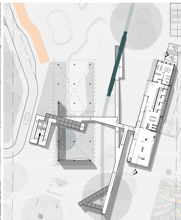
First Floor Plan scale 1:300
