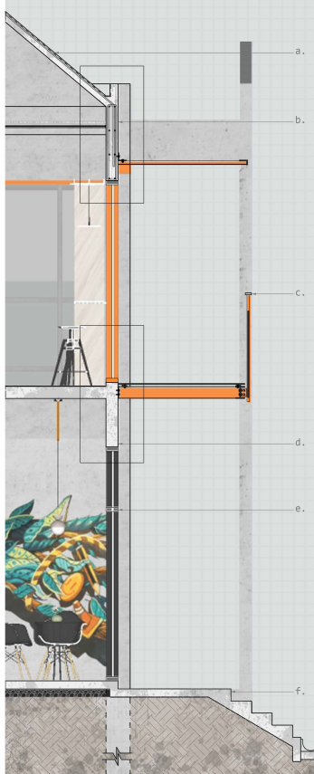
Sectional Detail scale 1:30
