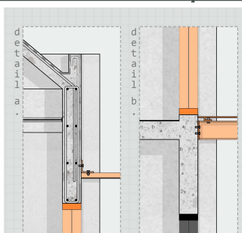
Blow-up Detail scale 1:15
