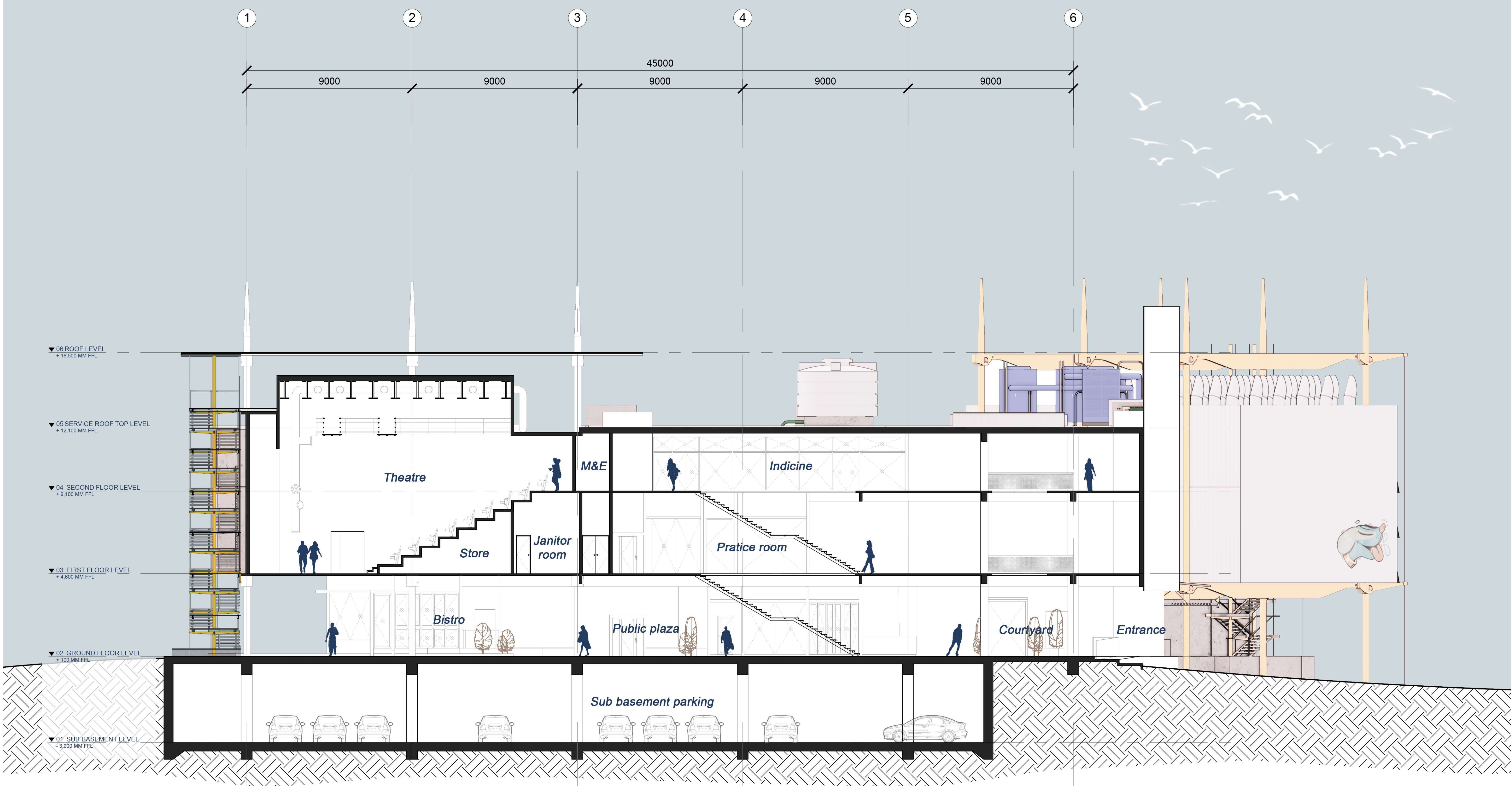
Section Y-Y scale 1:100
