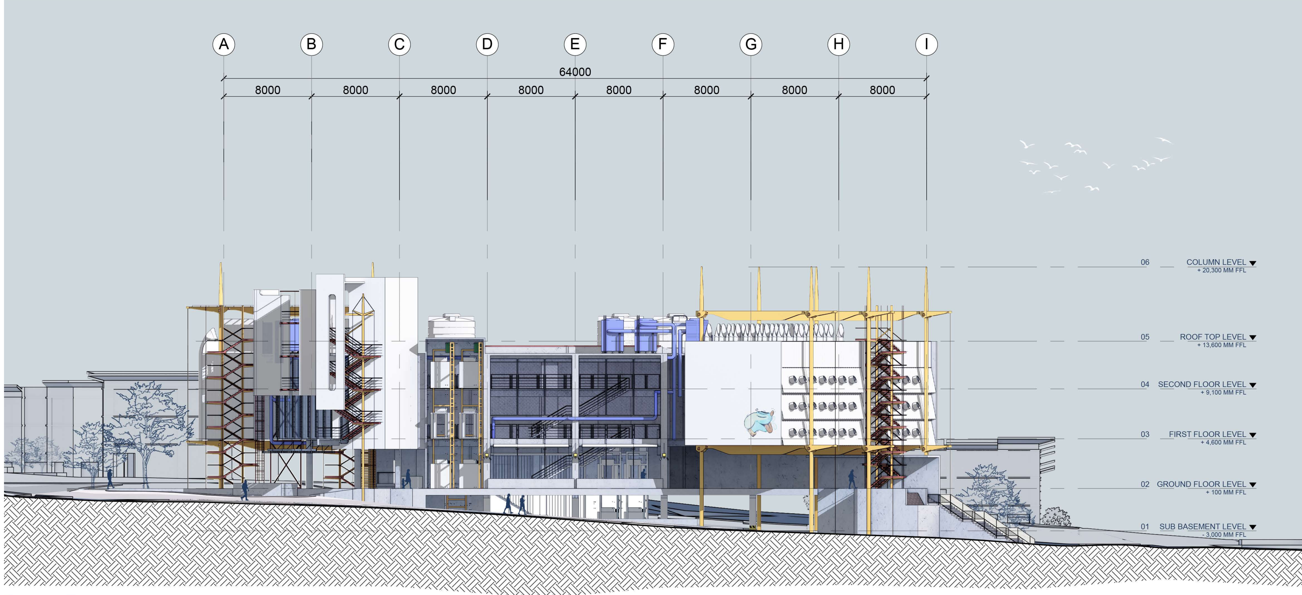
Right Elevation scale 1:200
