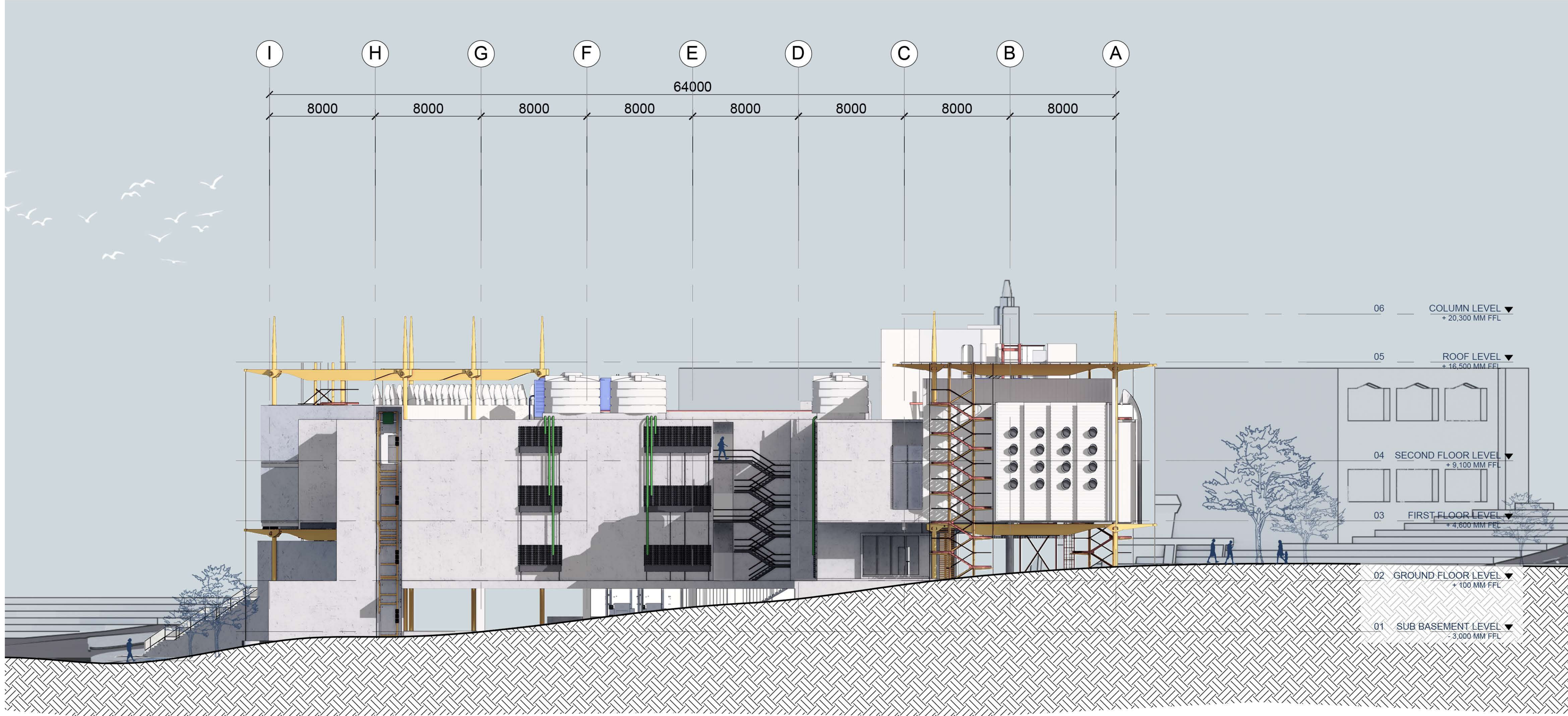
Left Elevation scale 1:200
