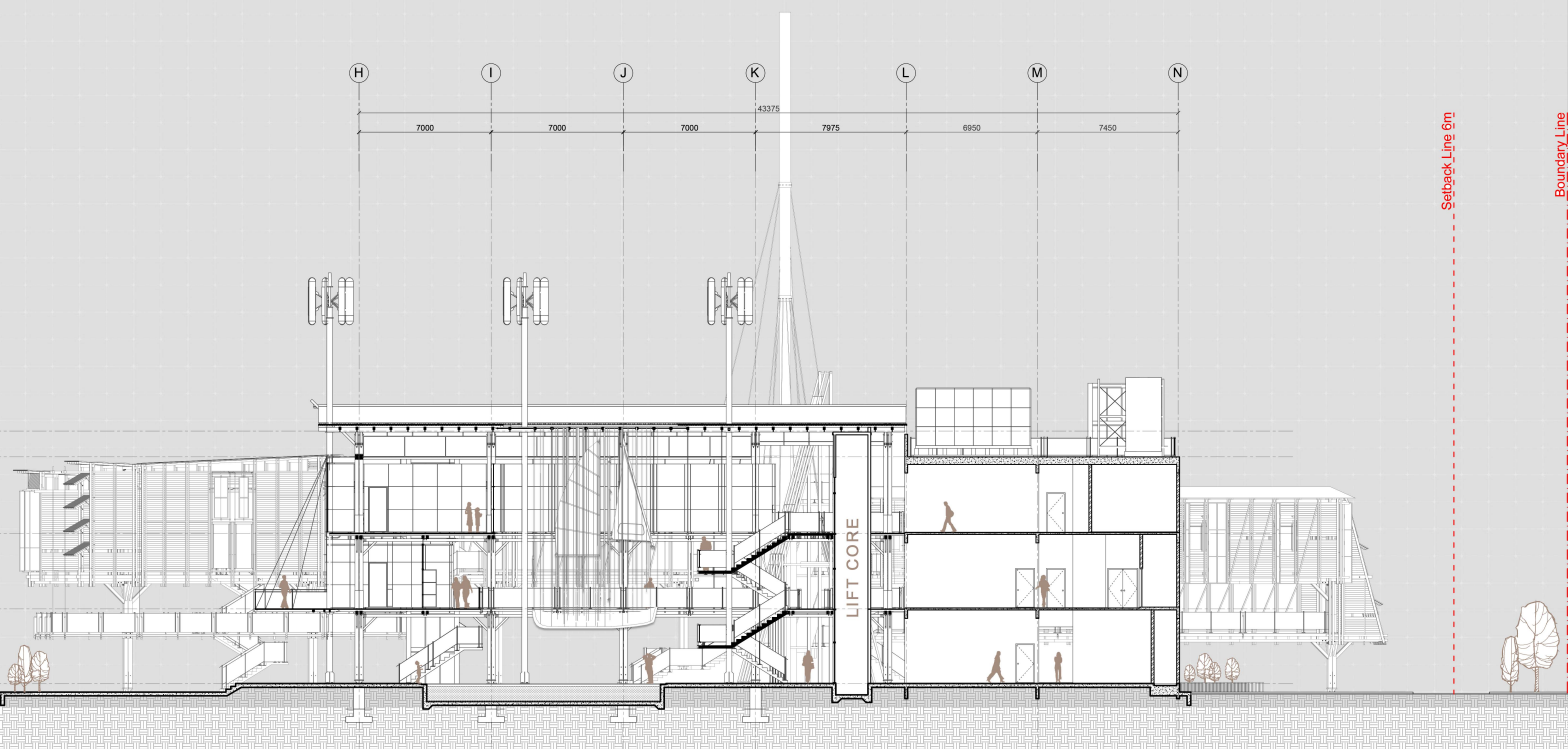
Section X-X scale 1:100
